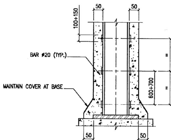
DETAIL AT COLUMN BASE
